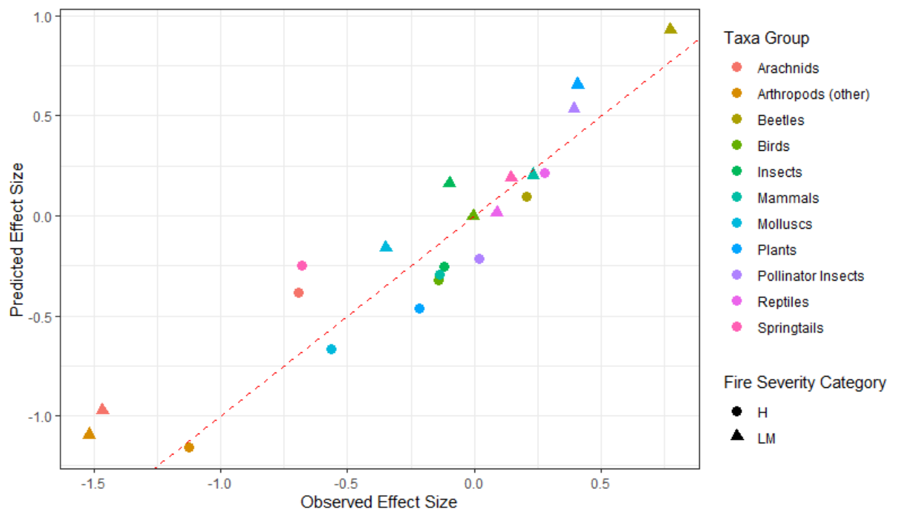
Figure C 11: Mean observed and model-predicted effect sizes by taxa group and fire severity. Note that the red dotted line indicates where observed = predicted, and if the points cluster around this equality, it can be interpreted that the predicted effect sizes are similar to the observed effect sizes, and thus the model is a good fit of the observed data.
