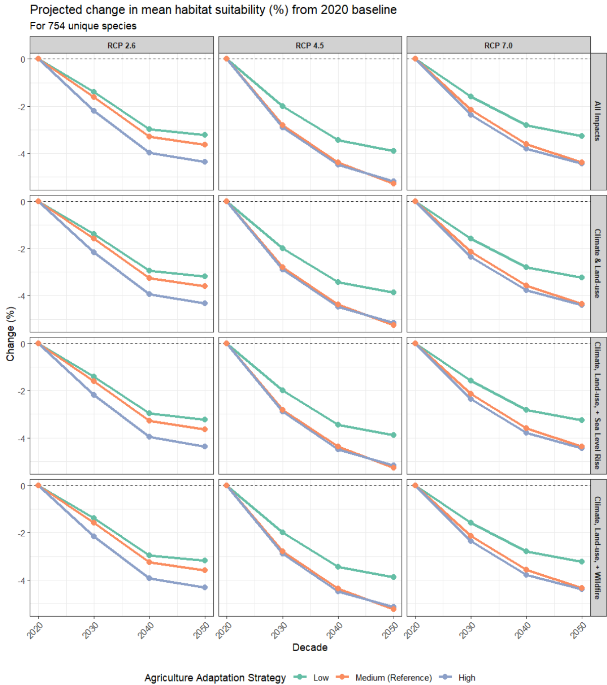
Figure E 2: Projected percent decadal change in mean suitable area for 754 species under different impacts (climate and land use only, with the addition of wildfire, with the addition of sea level rise, and all impacts combined); RCP(2.6; 4.5; 7.0) and adaptation scenarios (low, reference, high) from a 2020 decade baseline.
