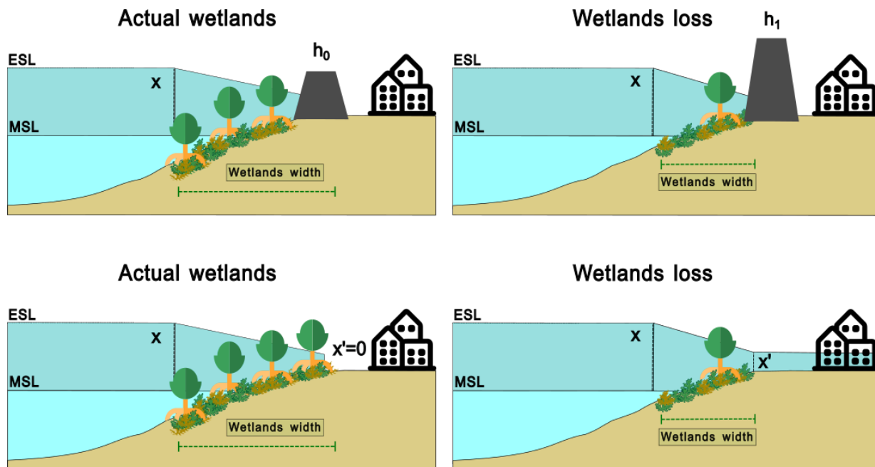
Figure 6: Avoided damage (lower panel) and replacement cost (upper panel) biophysical production function methods used for coastal wetlands coastal protection service valuation. In avoided damage the coastal protection benefit is framed as a reduction in expected annual damages from coastal flooding due to the presence of coastal wetlands on the floodplain. In replacement cost, the coastal protection benefit is framed as a reduction in the cost of building lower sea dikes (cost-saving) because the wetlands attenuate the water level.
