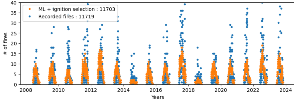
Figure C 5: Number of fires historically recorded (blue dots) per day. Number of fires obtained by our methodology using the fire risk maps from the ML model and our ignition selection method (orange dots). Note: We only focus on the fire season (June to October) hence the gaps between each year.
