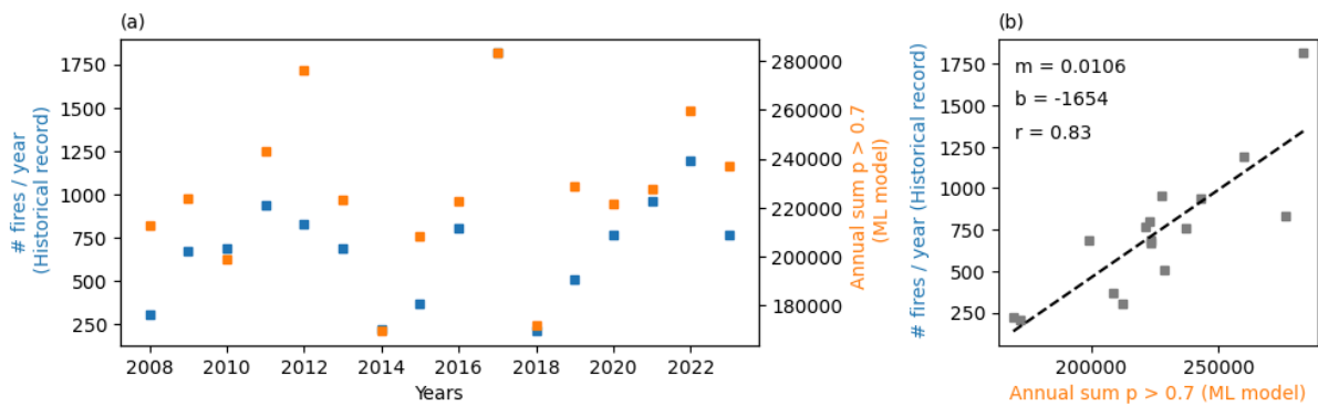
Figure C 4: (a) Historical record of fires (blue) and annual sum of the number of locations where p > 0.7 from the ML model (orange); (b) Same as (a) but one against the other.
