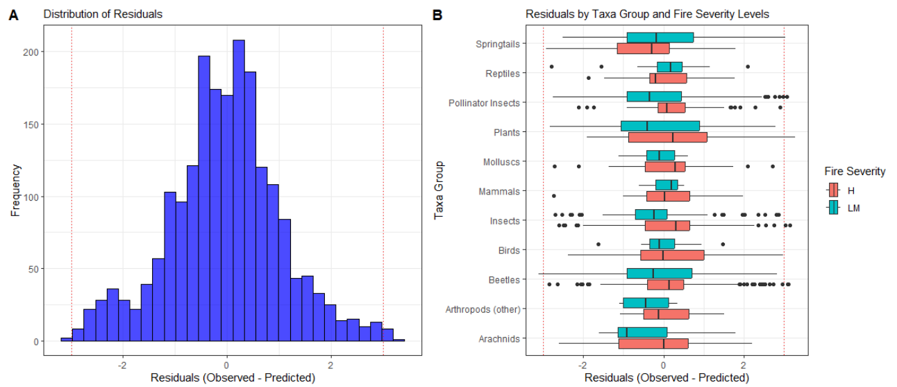
Figure C 13: Overall distribution of effect size residuals (observed – predicted) to show the distribution of model prediction errors. (B) Distributions of effect size residuals (observed – predicted) by taxa group and fire severity to show the distribution of model prediction errors.
