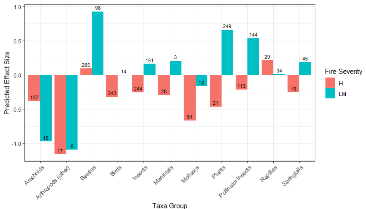
Figure C 12: Mean predicted effect size by taxa group and fire severity. The numbers on each bar indicate the number of observed effect sizes used to calculate the mean predicted effect size.
