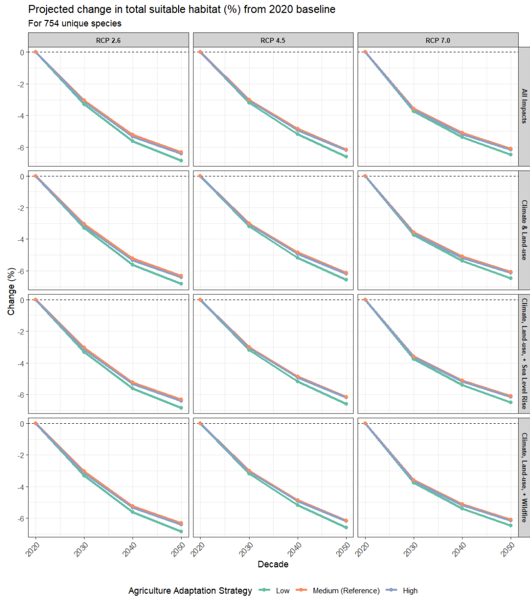
Figure E 1: Projected percent decadal change in total suitable area for 754 species under different impacts (climate and land use only, with the addition of wildfire, with the addition of sea level rise, and all impacts combined); RCP(2.6; 4.5; 7.0) and adaptation scenarios (low, reference, high) from a 2020 decade baseline.
