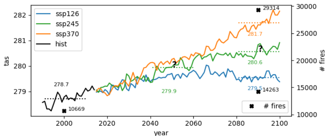
Figure C 7: The colored lines represent the evolution of the global mean surface temperature for the different climate scenarios. The crosses (x) are the predicted number of fires under the different scenarios for the Mediterranean region.
