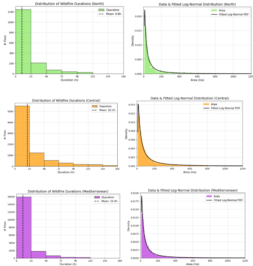
Figure C 9: historical distribution of fire duration and size. Green (North), orange (Central), pink (Mediterranean)
