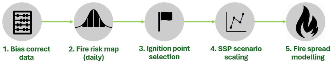
Figure C 1: Overview of DTU wildfire modeling methodology.
