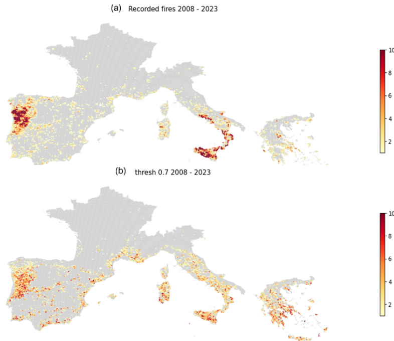
Figure C 6: Number of fires per grid cell (a) from the historical record (b) from the ML probabilities using ERA5-land
