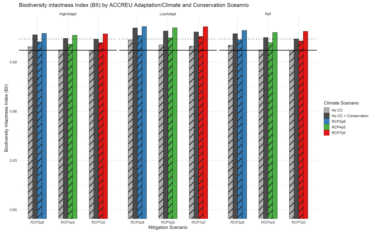
Figure 20: Biodiversity Intactness Index (BII) in 2050 for Europe under combined adaptation, conservation, climate, and mitigation scenarios using the ACCREU framework. Bars represent BII outcomes for different mitigation pathways (RCP2.6, RCP4.5, RCP7.0) across adaptation scenarios (High Adaptation, Low Adaptation, Reference Adaptation). Bar colors indicate climate impact scenarios, while hatching indicates scenarios with the absence of conservation and restoration actions. The solid black lines indicate the baseline BII for the scenario with reference adaptation, reference climate and no mitigation and no conservation), while the dotted green lines show the BII for the same scenario but with conservation policy.
