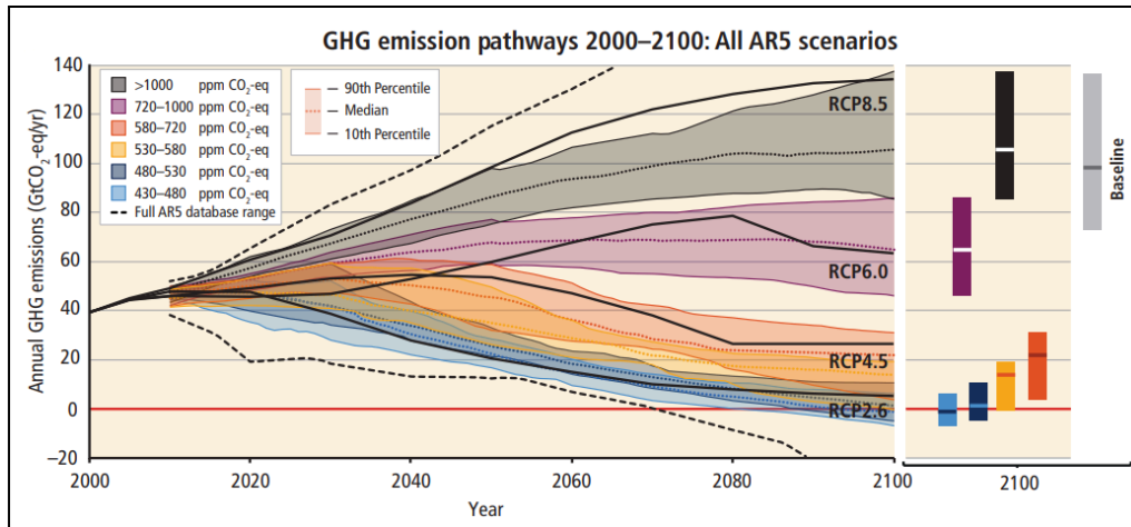
Figure 2 | Emission from different RCPs Source: IPCC AR5, SPM (2014).
