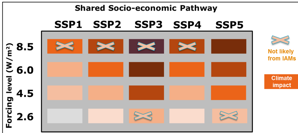
Figure 3 | Feasibility of alternative forcing agents across the SSPs. Source: our elaboration based based on Riahi et al. (2017)
