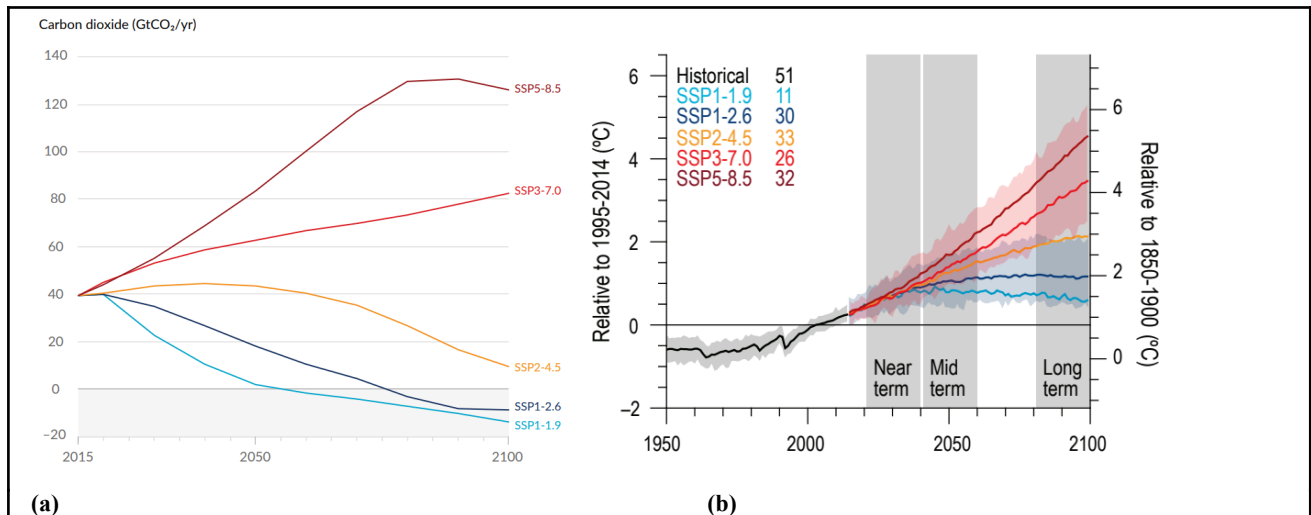
Figure 4 | Annual CO 2 emissions (a) and relative global surface air temperature changes (b) for selected SSP-RCP combinations. Source: IPCC AR6, 2021, pp. 571 (a) and pp. 13 (b)
